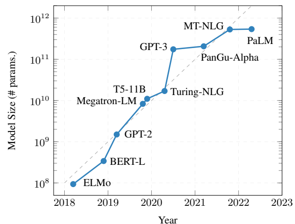
Figure 1: Evolution of the size of large pretrained language models. Adapted from Lakim et al. (2022).
